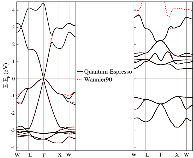
Majority-spin
