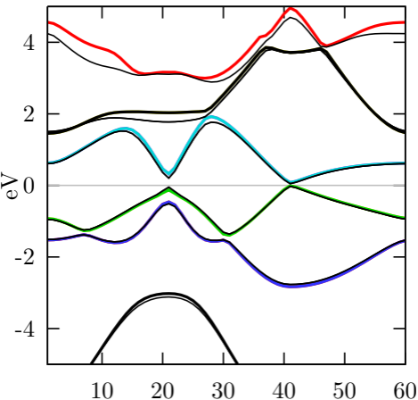
Statene Band Structure w ESPRESSO NCP (color) vs PAW (thin-black), w SOC
