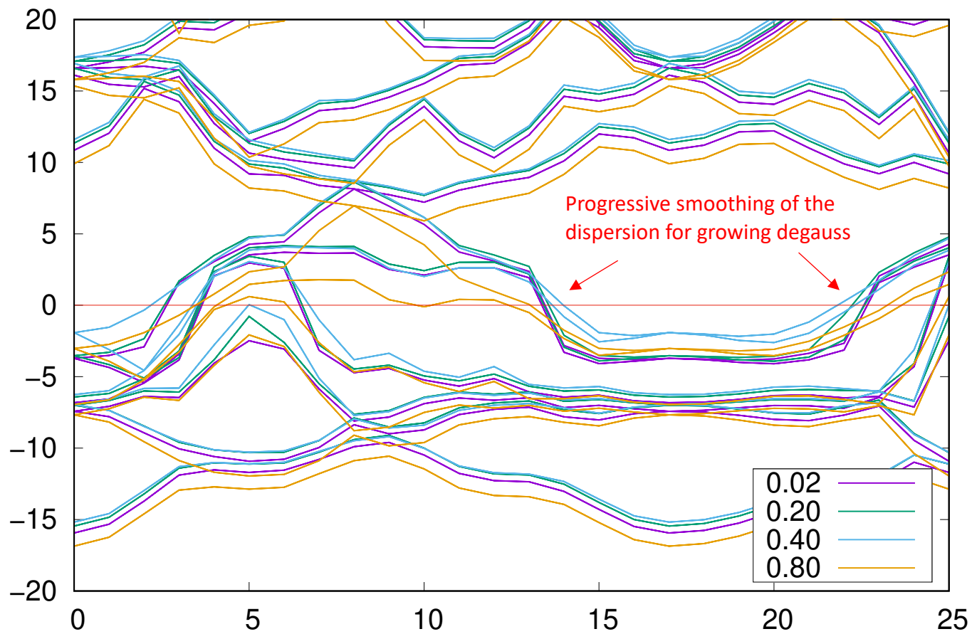
regular kpt grid = 8 \times 8 \times 8 ; varying DEGAUSS
