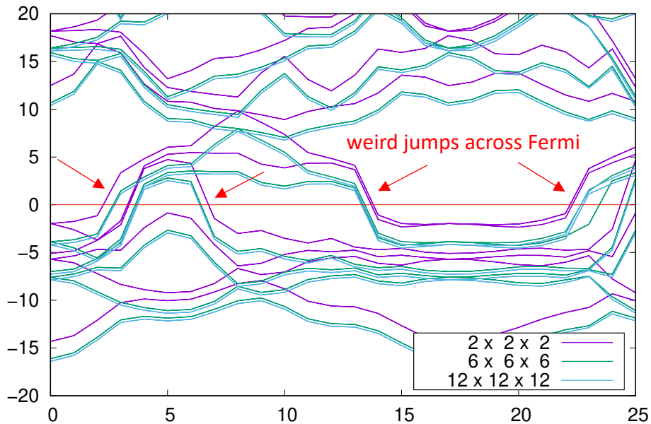
DEGAUSS = 0.02 ; varying regular kpt grid
