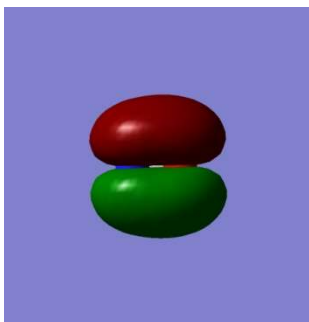
1π orbital (any other codes)
