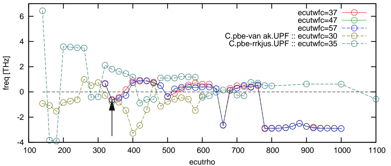
single q-calculation :: q=(0,0.01,0) :: C.pbe-n-rrkjus psl.0.1.UPF :: tr2 ph test
