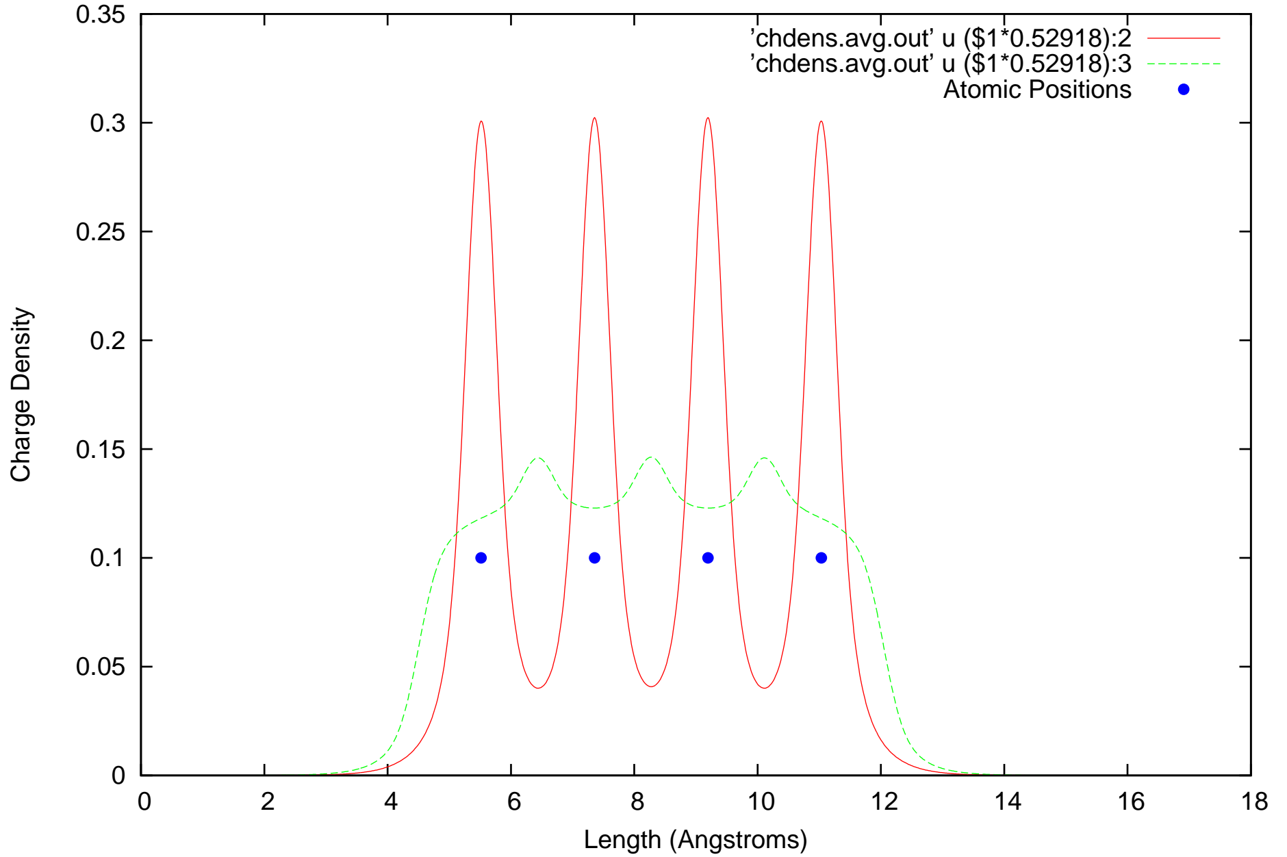
Cu100 PP-van-ak
