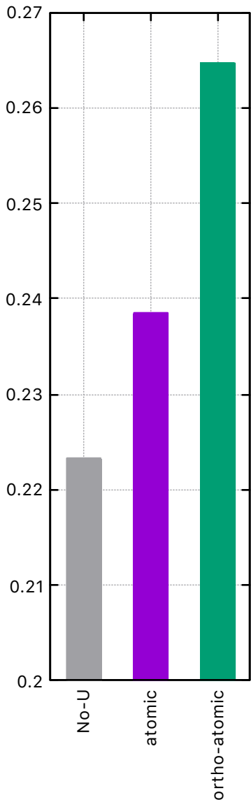
Path integral
